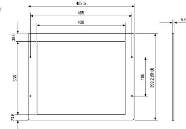
19"-Einbaukit / 19" Rack mount kit
